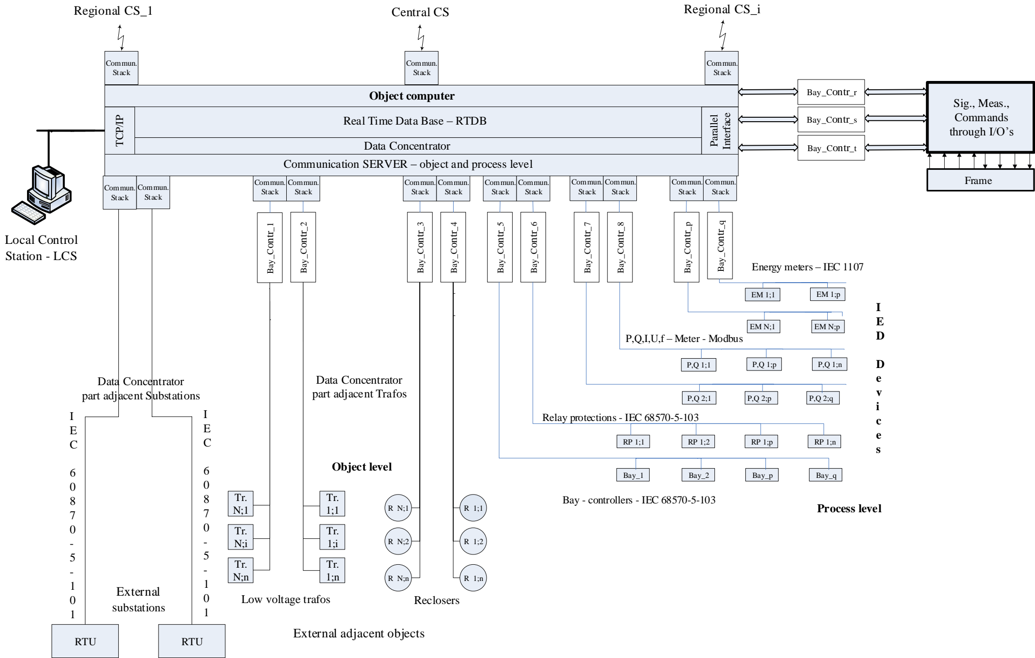
Decentralized RTU
