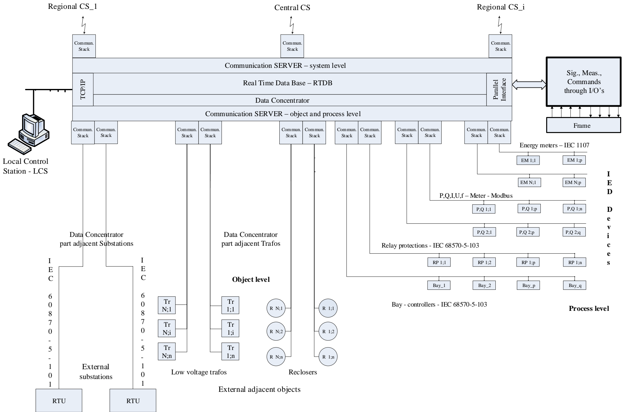
Centralized RTU
